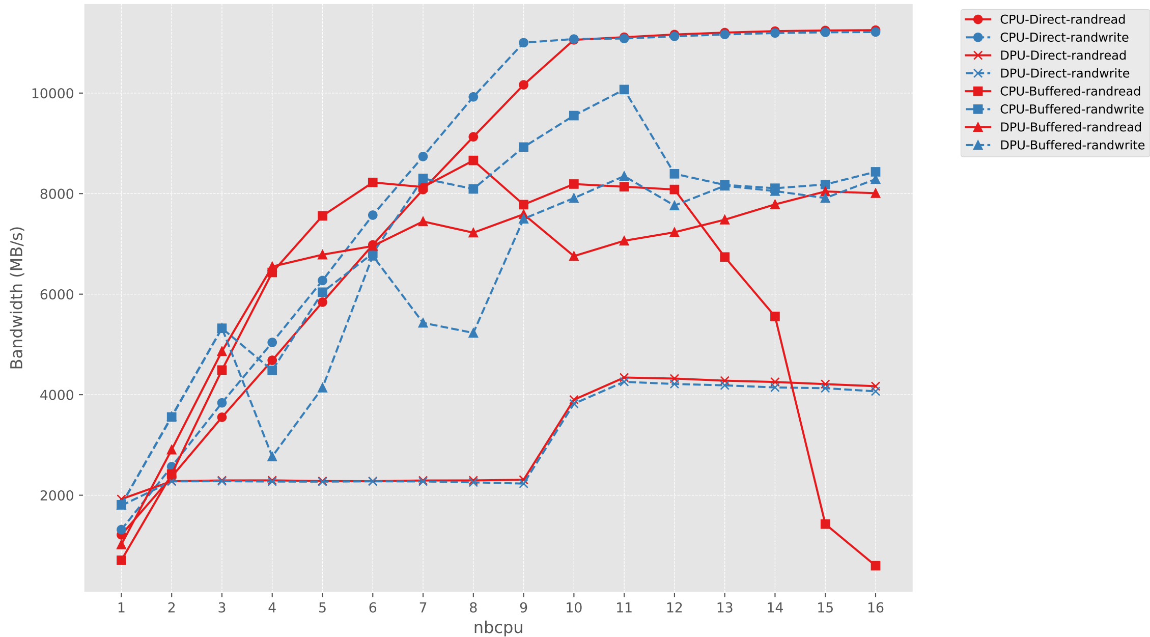
Bandwidth vs nbcpu (CPU vs DPU, Direct vs Buffered)
